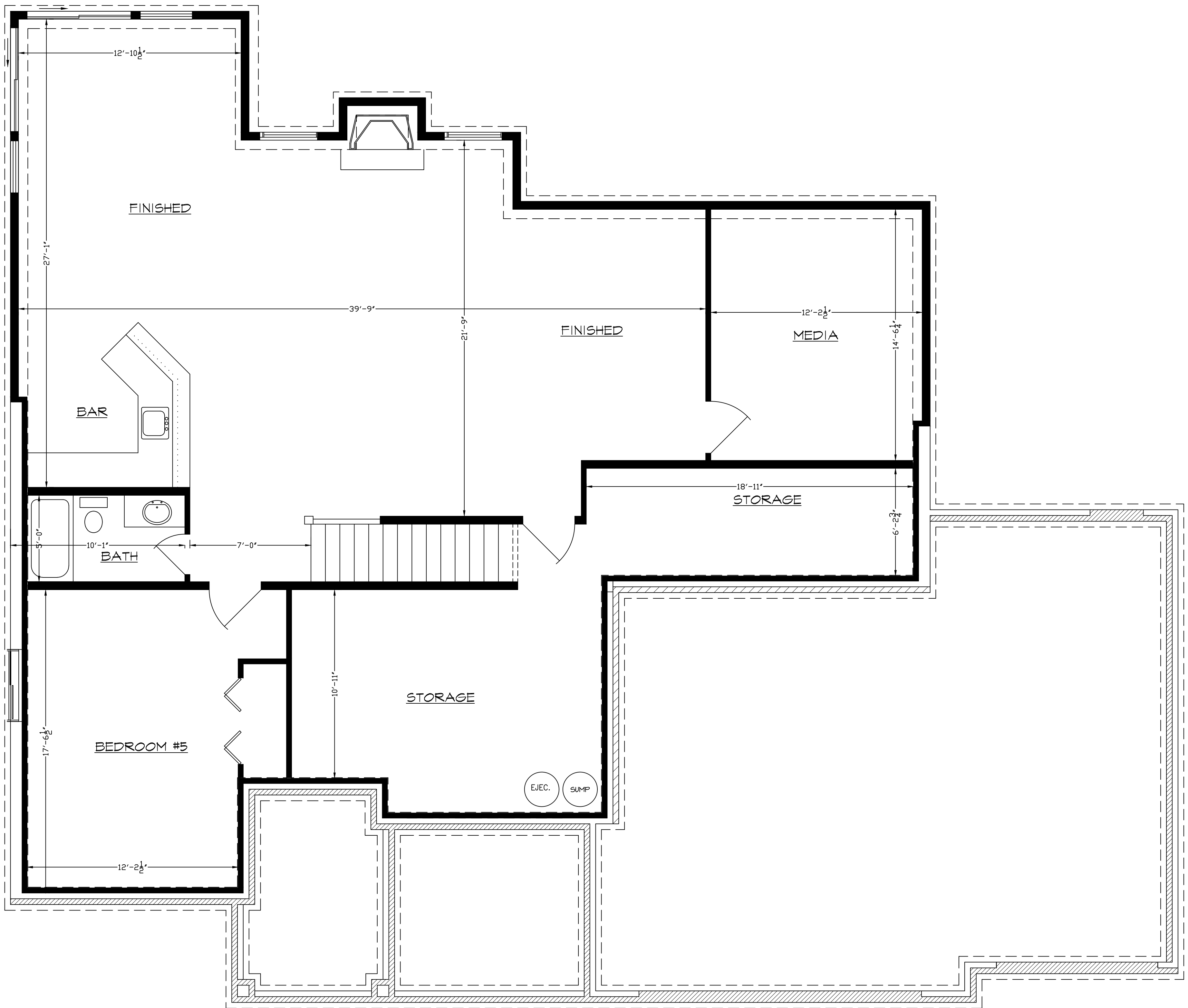
BASEMENT 1457 SQ. FT. FINISHED
