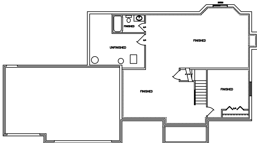
FINISHED BASEMENT 1,055 SF (OPTIONAL)
